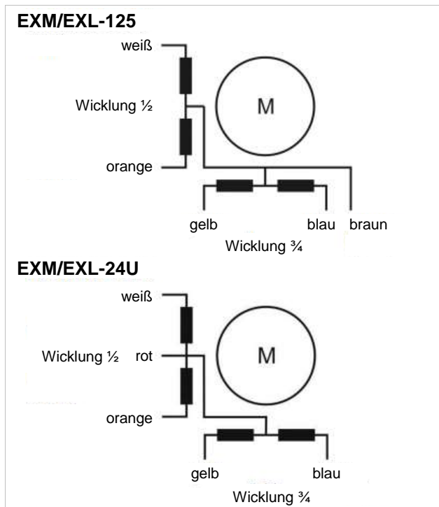
Abb. 14-1 – Expansionsventile
